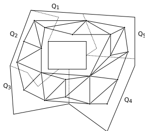
Figure 2: An example of a maximal partial triangulation within a DP cell and a partition of the DP cell into smaller DP cells Q_1, \dots, Q_5 crossing some triangles in the triangulation.
